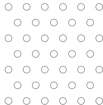
R18-216SG13 1/8" HOLES ON 21/64" STAGGERED CENTERS 13% OPEN AREA
